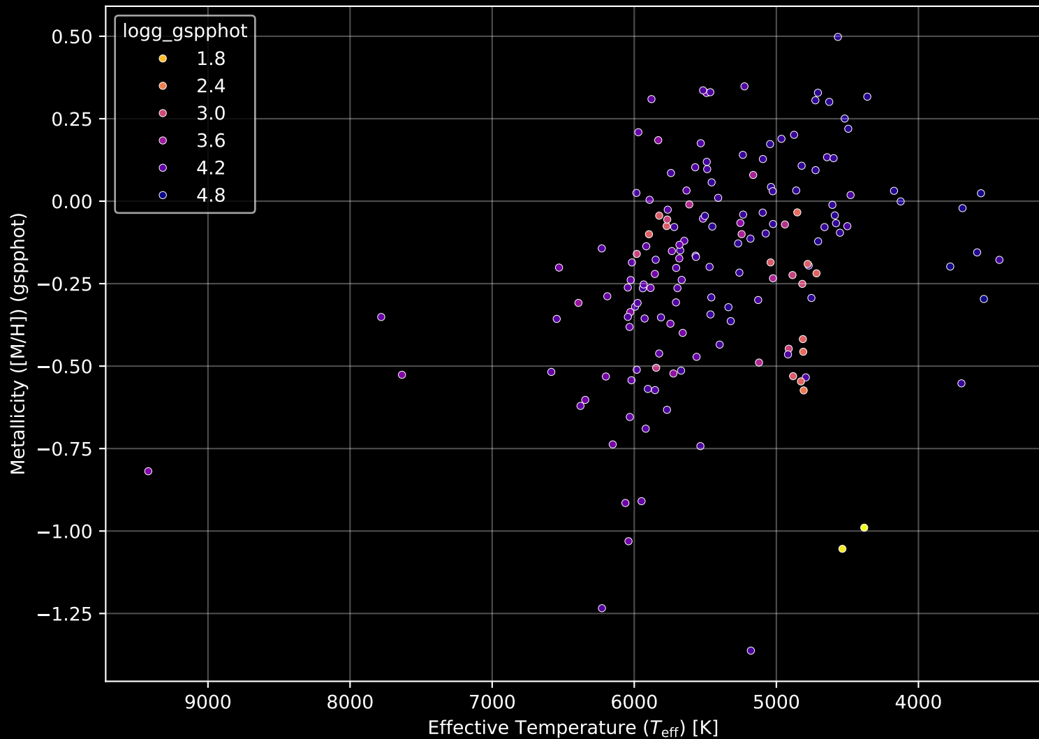
APOGEE DR17 Field: [149+59_MGA] Stellar Population Parameters (n= 162)
