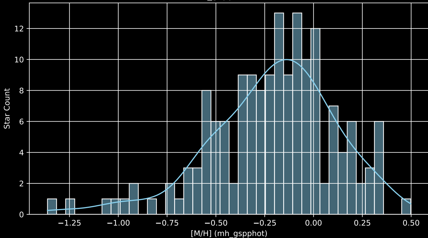
APOGEE DR17 Field: [149+59_MGA [M/H] (mh_gspphot) (n= 162)
