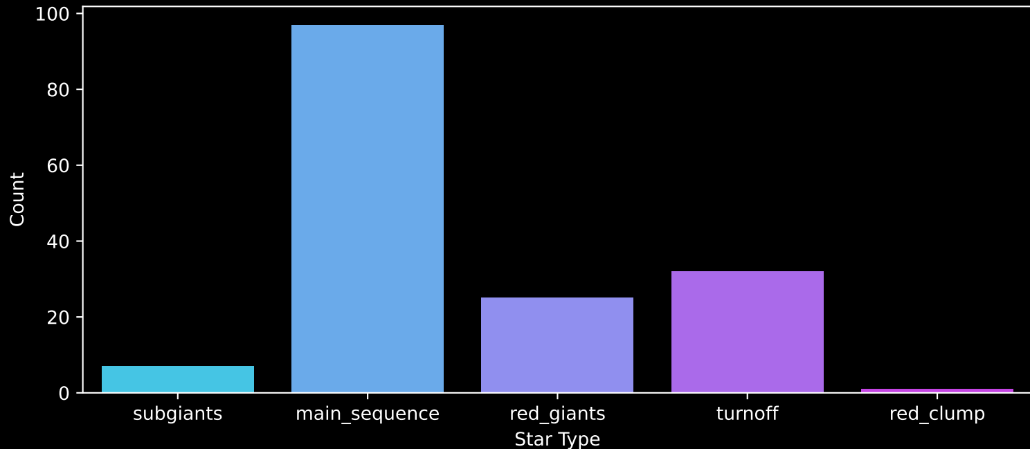
APOGEE DR17 Field: [149+59_MGA] Count plot of Star Type
