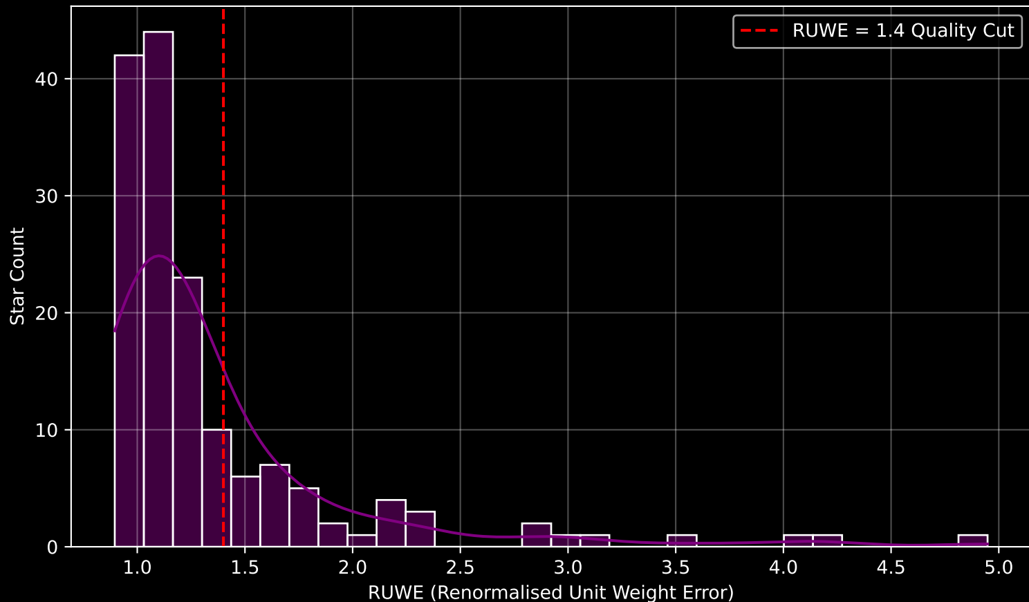
GAPOGEE DR17 Field [149+59_MGA] RUWE Distribution (n= 155)
