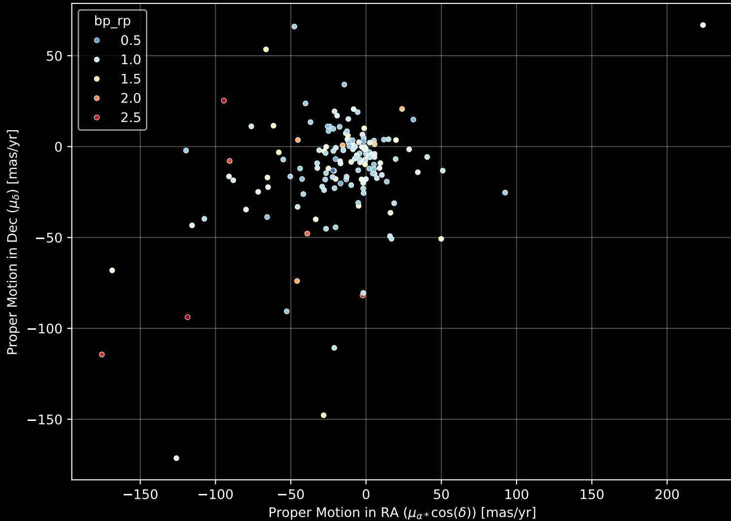
APOGEE DR17 Field: [149+59_MGA] Proper Motion Diagram (n= 162)
