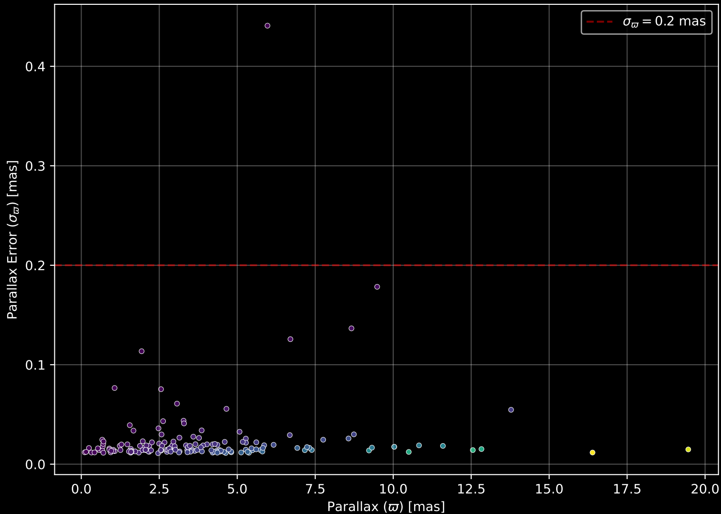
APOGEE DR17 Field: [149+59_MGA] Parallax Quality (n= 162)
